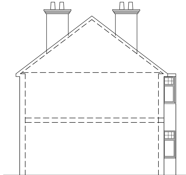
PARTY WALL ELEVATION
