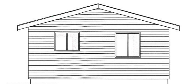
Front Gable Elevation
