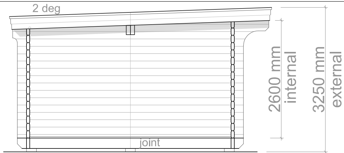
North Elevation
