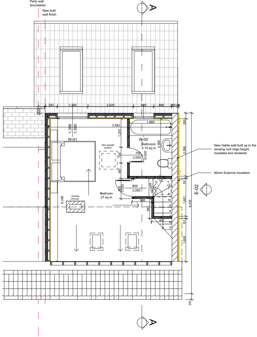
SF 02 Proposed Second Floor Plan 1:100
