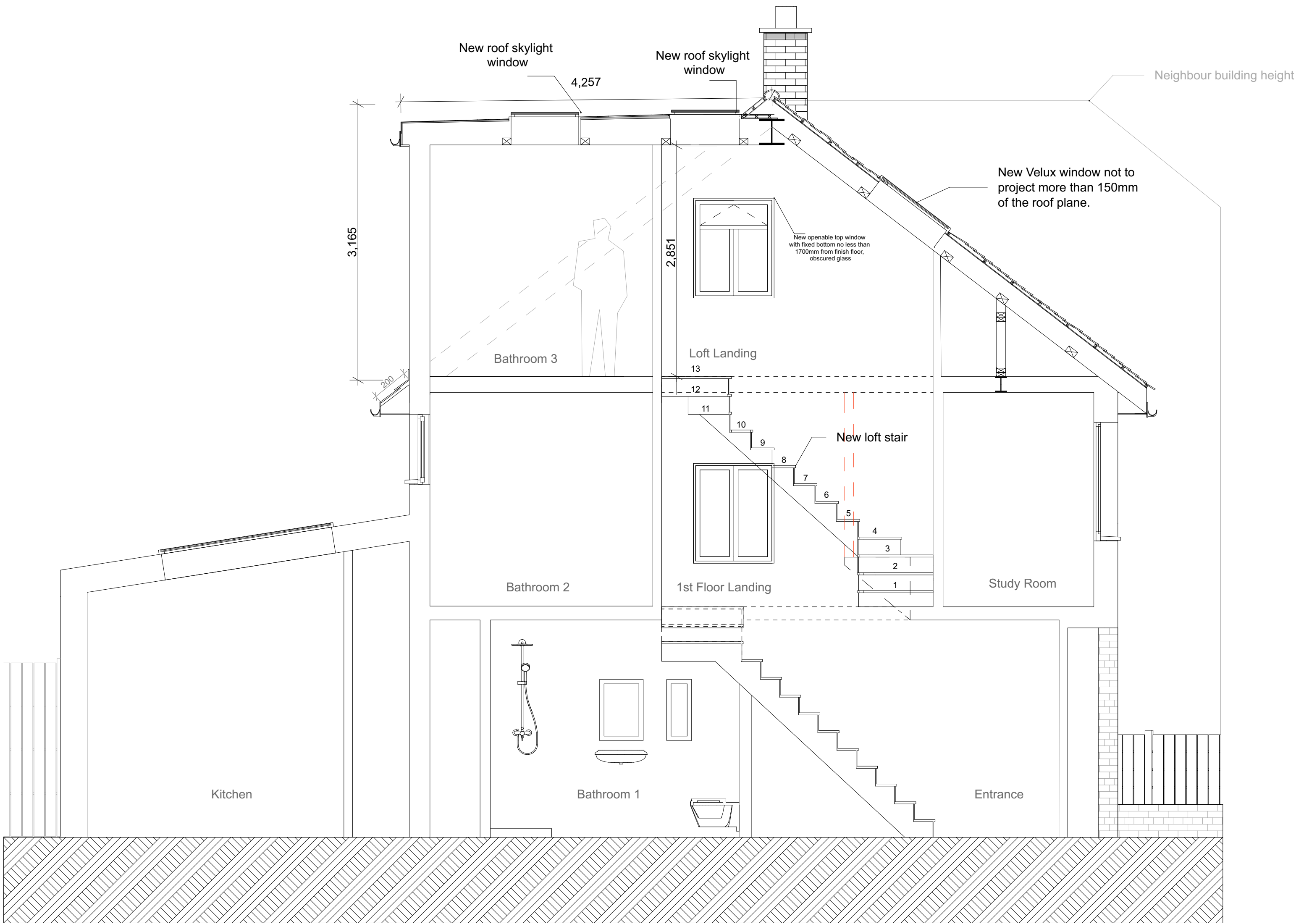
S 01 Proposed Section A 1:50
