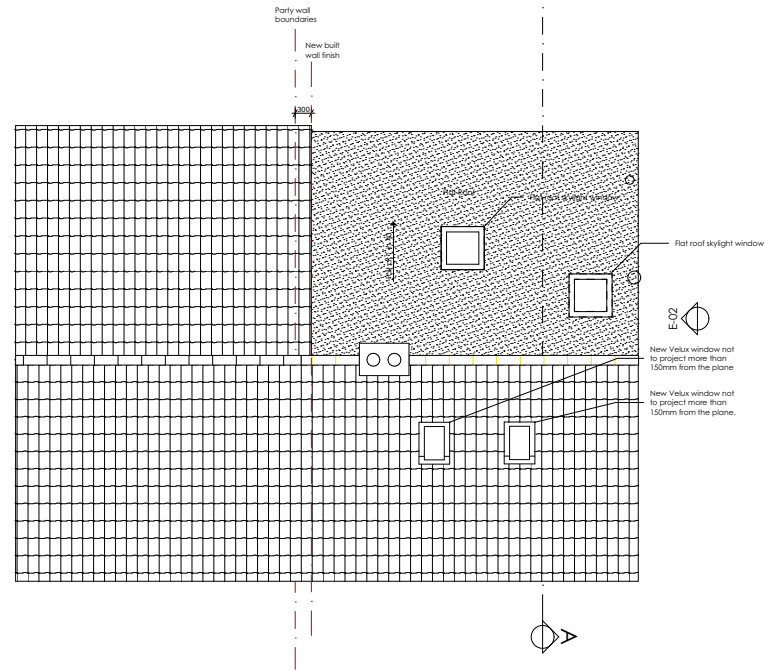
RF 02 Proposed Roof Plan 1:100
