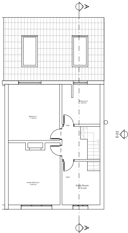
FF 01 Existing First Floor Plan 1:100
