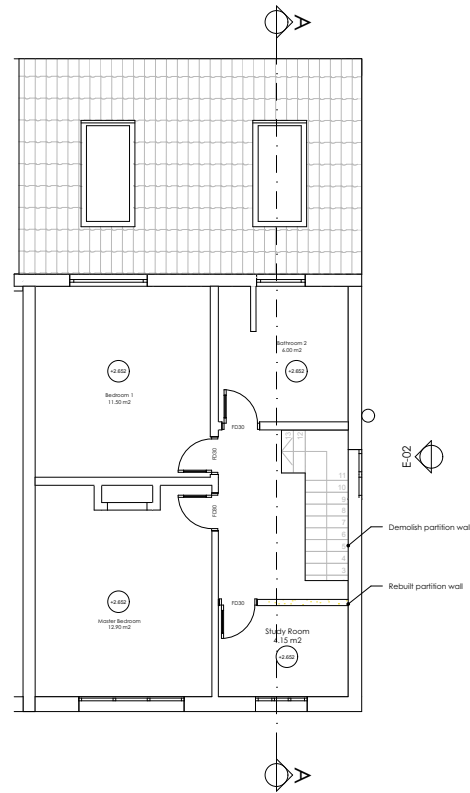
FF 02 Proposed First Floor 1:100
