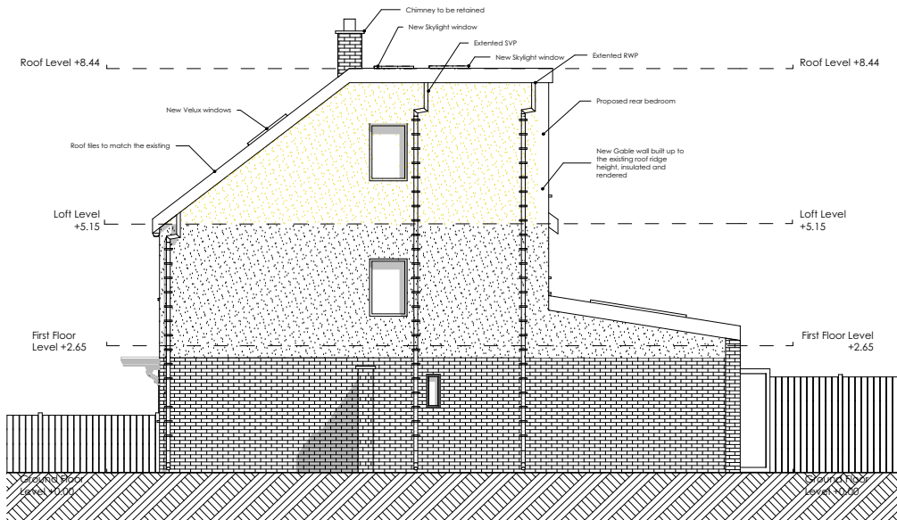
E 02 Proposed side elevation 1:100
