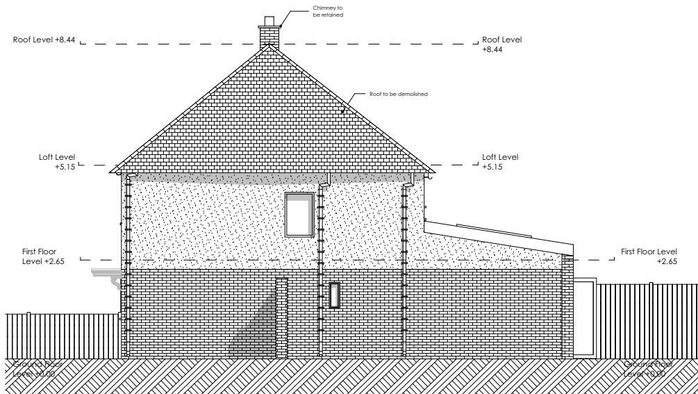
E 01 Existing side elevation 1:100
