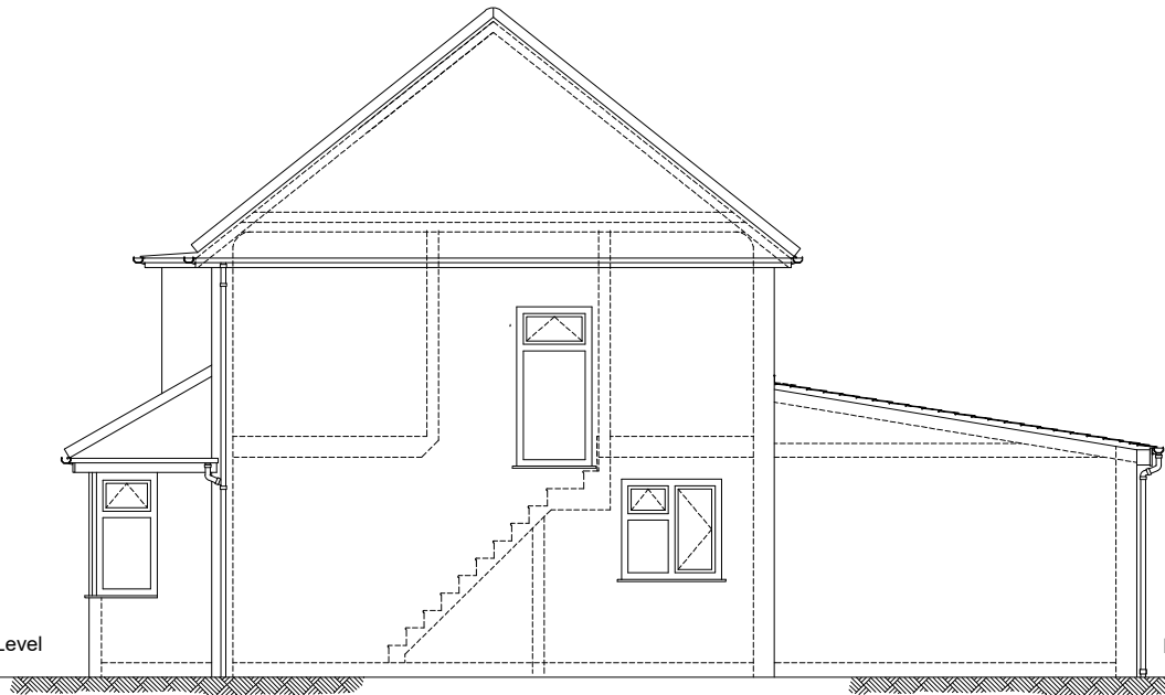
Existing Side Elevation (C-C)
