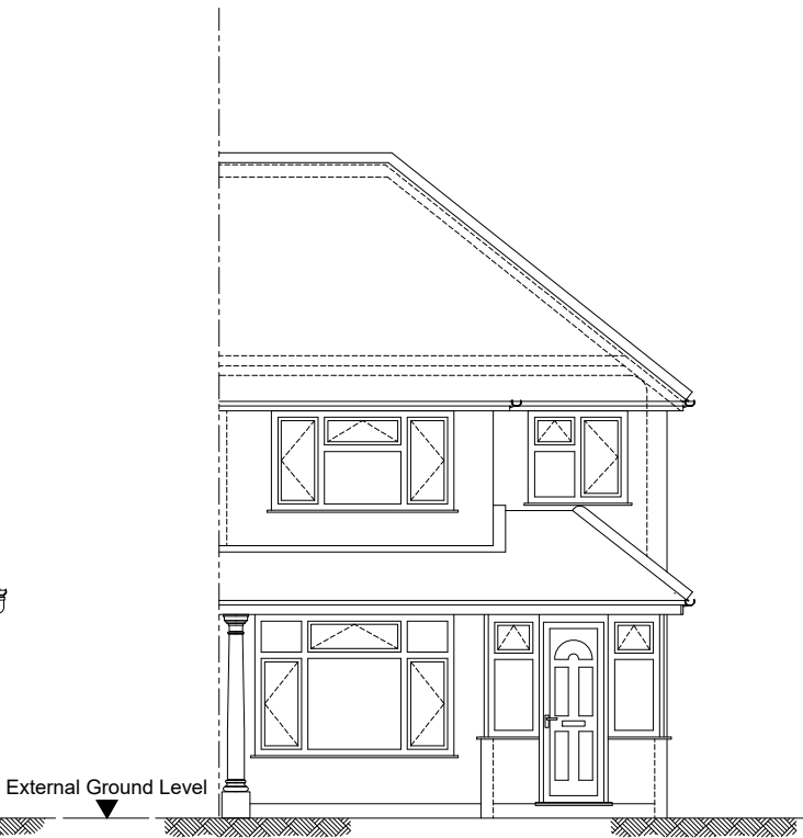
Existing Front Elevation (A-A)
