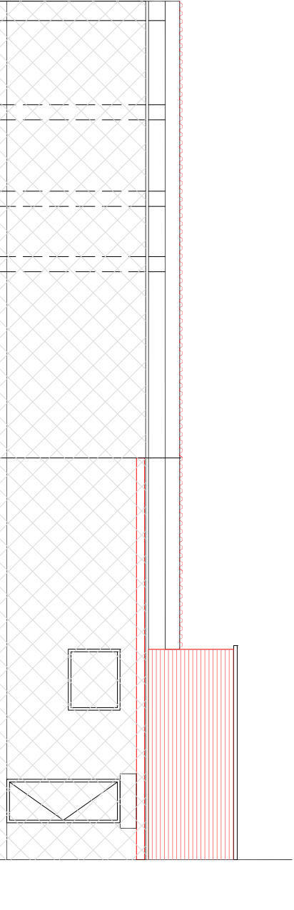
EXISTING SIDE ELEVATION FROM SIDE ACCESS
