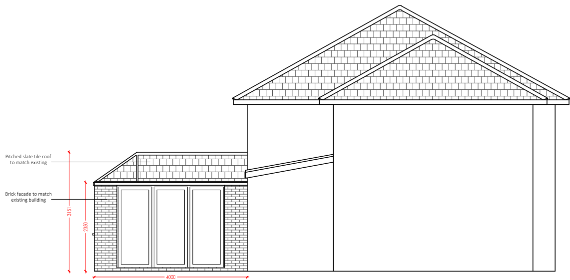
PROPOSED SOUTH FACING ELEVATION
