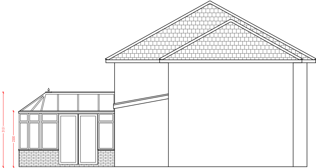
EXISTING SOUTH FACING ELEVATION
