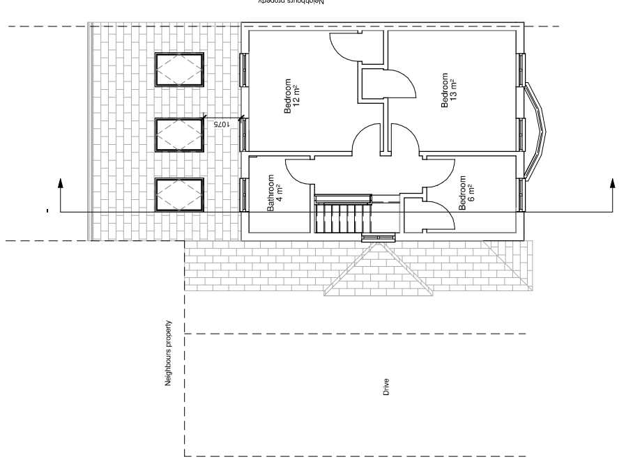
01-First floor - Proposed 1 : 100
