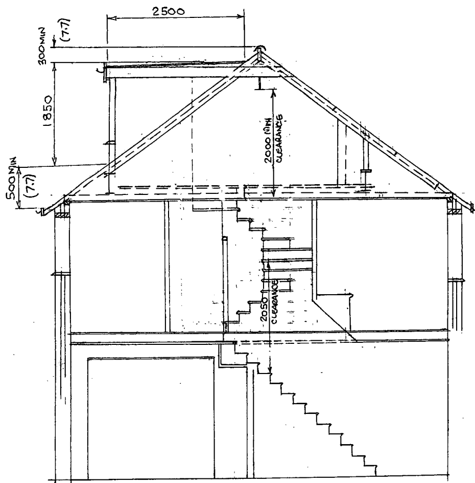
SECTION THROUGH STAIRCASE.
