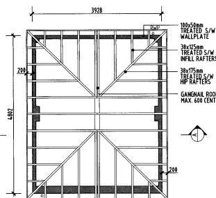
ROOF PLAN
