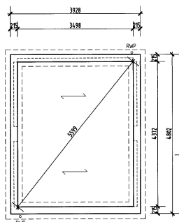
FOUNDATION PLAN
