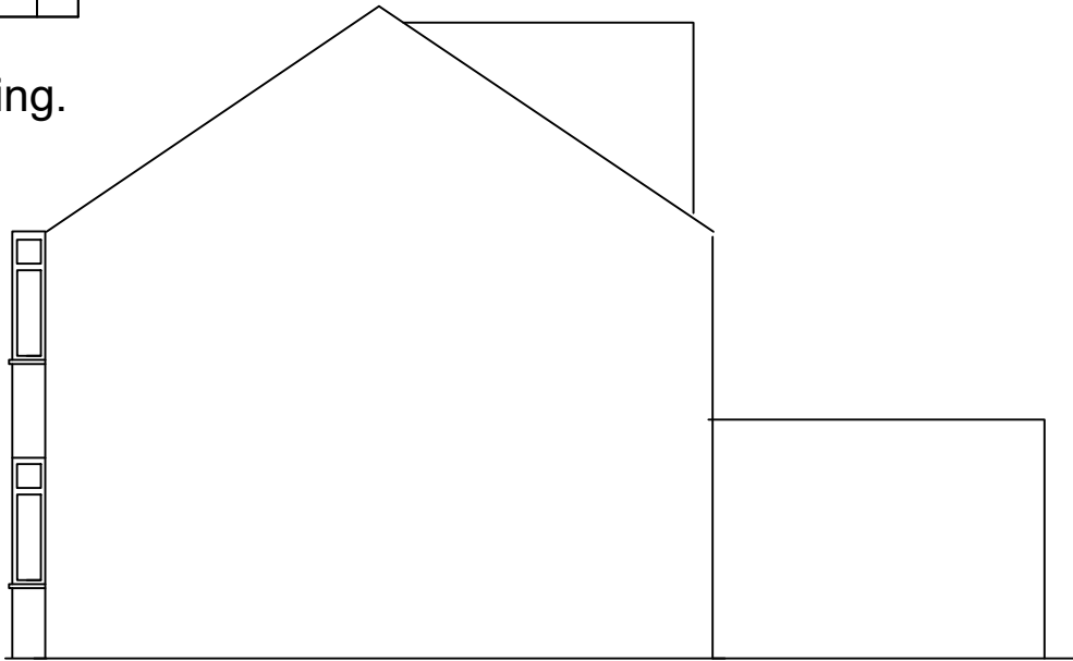
Proposed Side Elevation View From No.35
