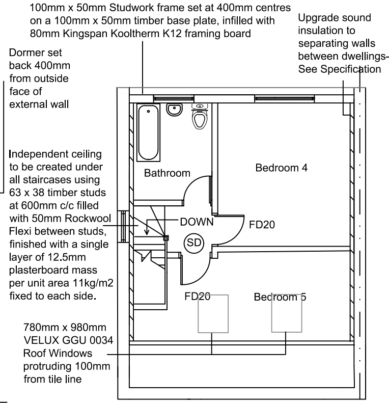
Proposed Loft Floor Plan
