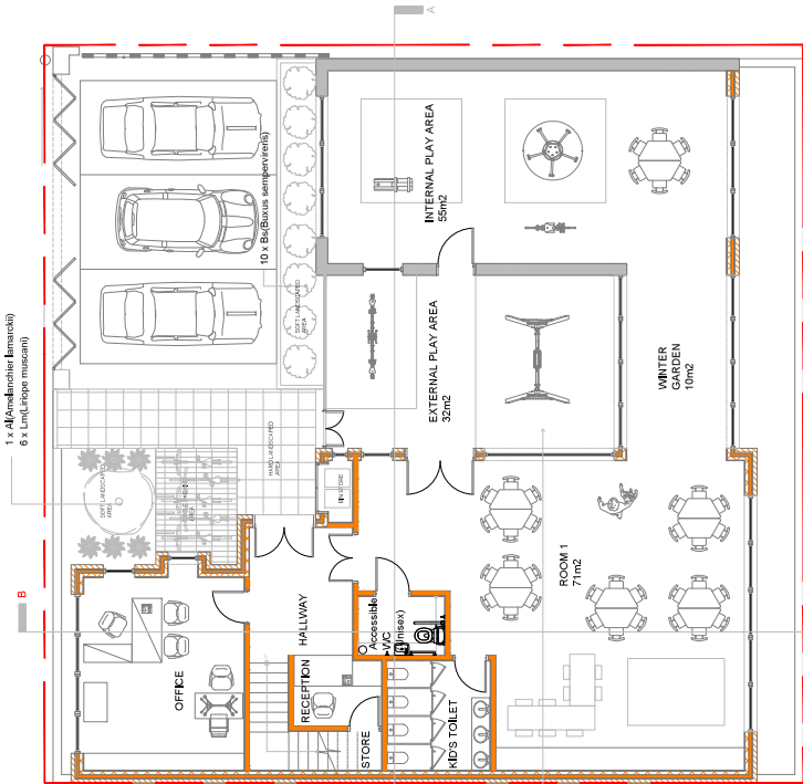
PROPOSED FLOOR PLAN - GROUND FLOOR
