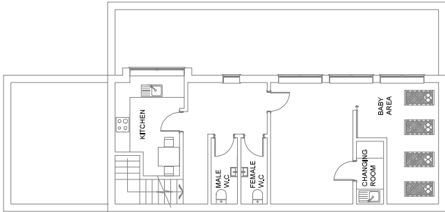
APPROVED FLOOR PLAN-FIRST FLOOR (62125/APP/2018/3118)
