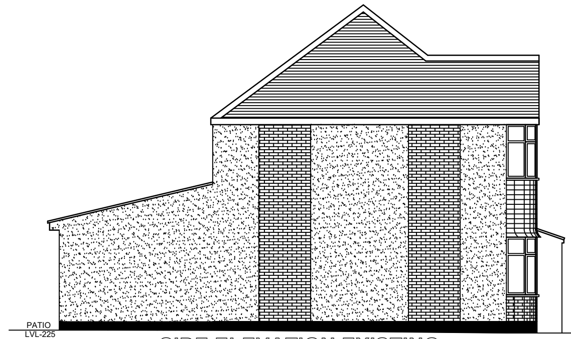
SIDE ELEVATION EXISTING (AS VIEWED FROM NO.66)
