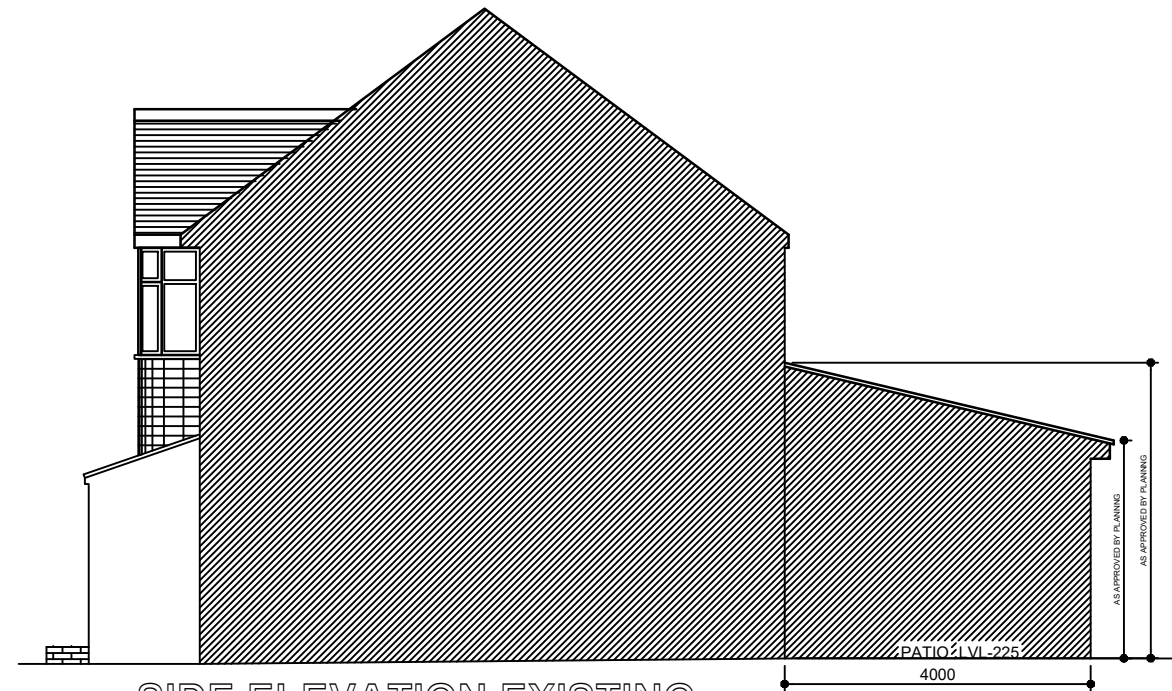
SIDE ELEVATION EXISTING (AS VIEWED FROM NO.62)
