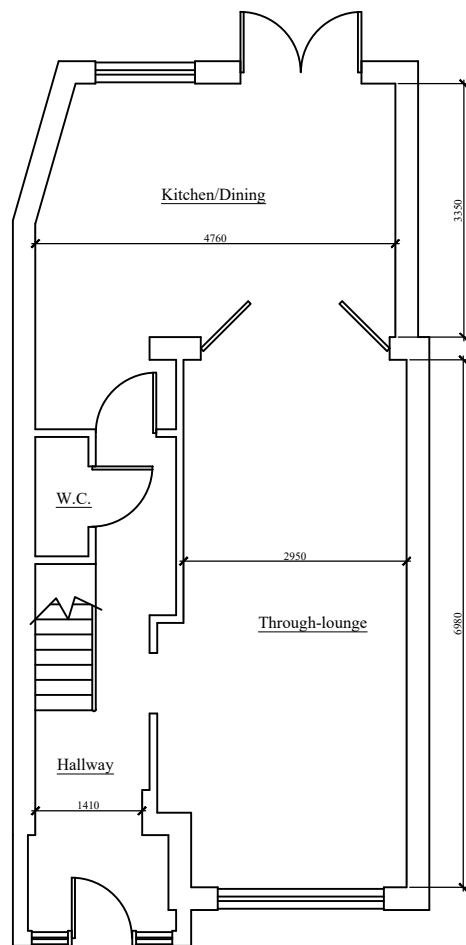
4 Seaton Road - Former Ground Floor Layout
