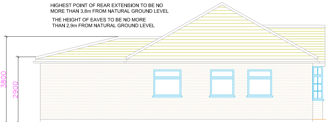
PROPOSED SIDE ELEVATION-2
