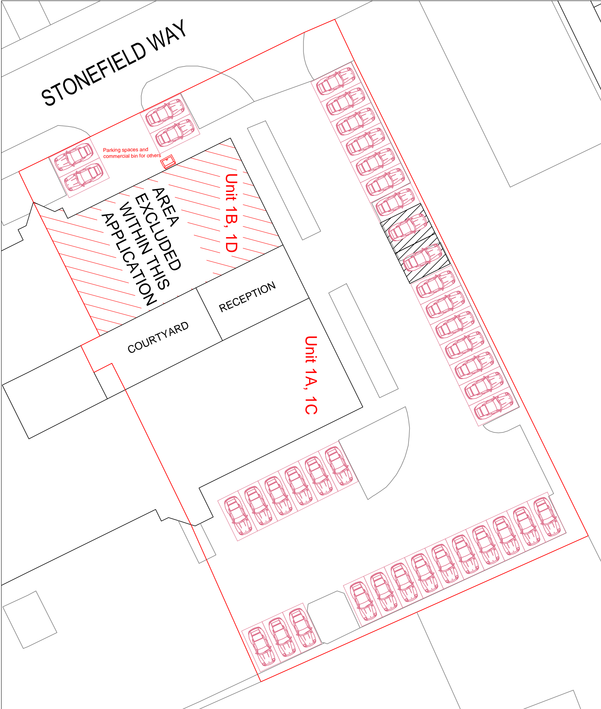
BLOCK PLAN (CAR PARKING) Scale 1:250
