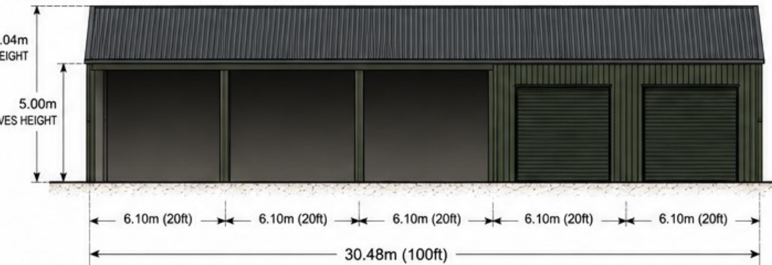
WEST ELEVATION (SIDE)
