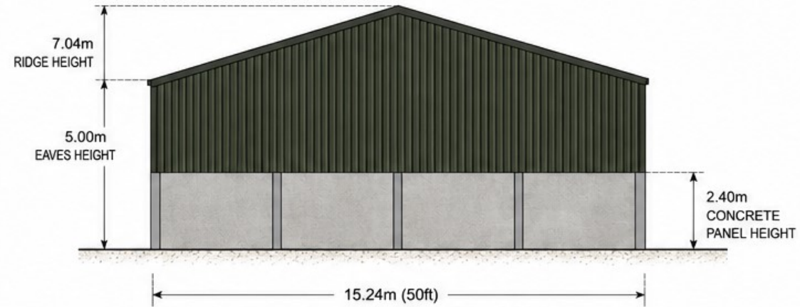
NORTH ELEVATION (GABLE END)
