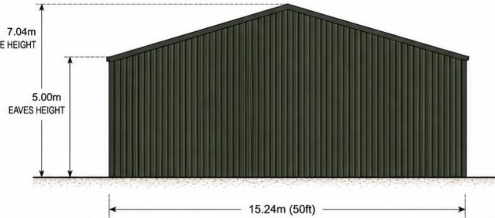
SOUTH ELEVATION (GABLE END)
