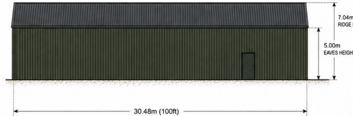
EAST ELEVATION (SIDE)
