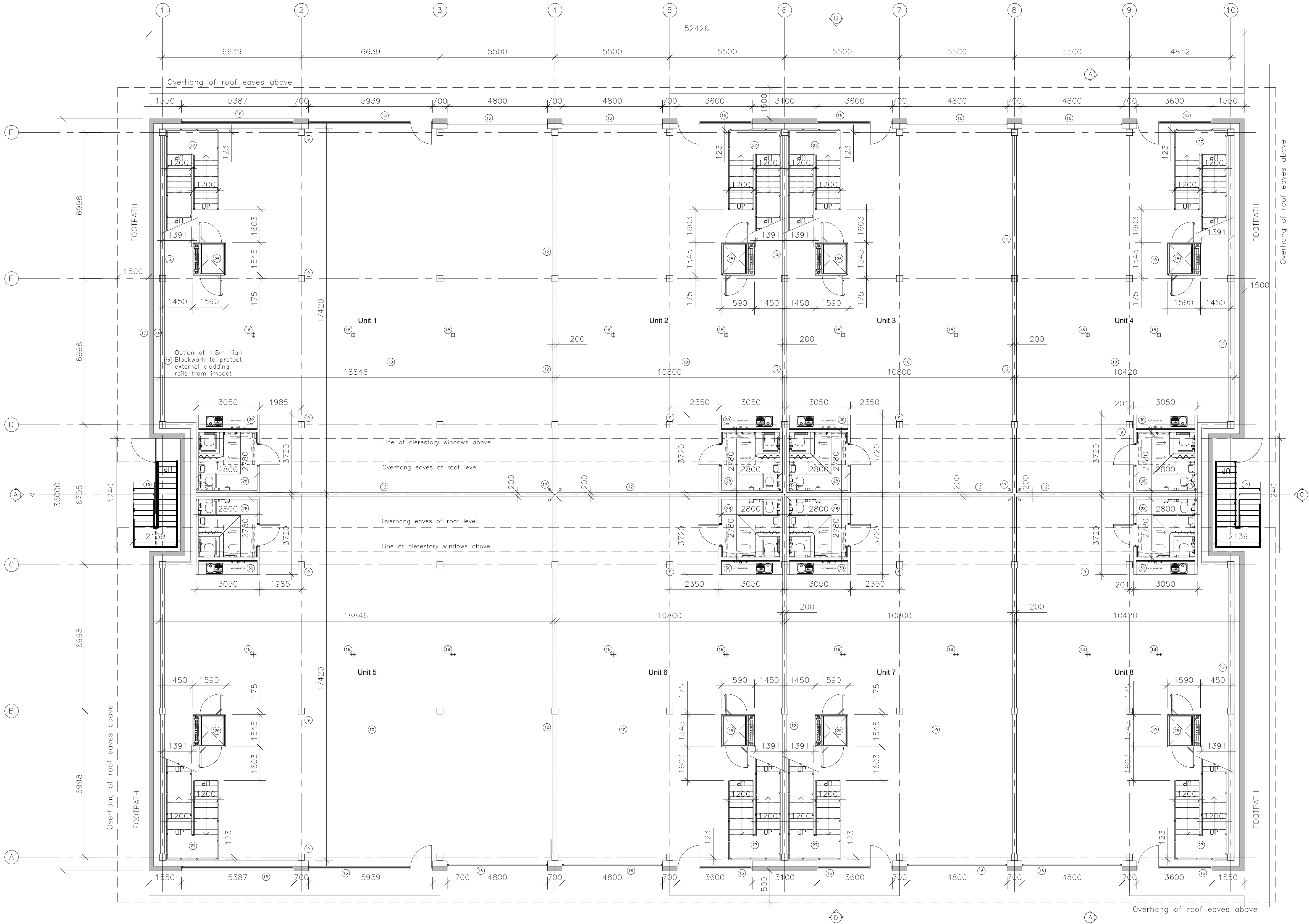
Building A Ground Floor General Arrangement
