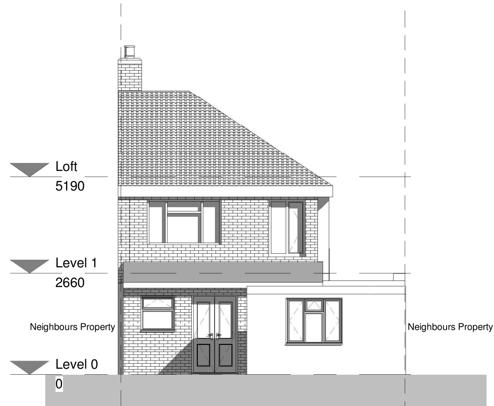
Rear elevation - Existing
