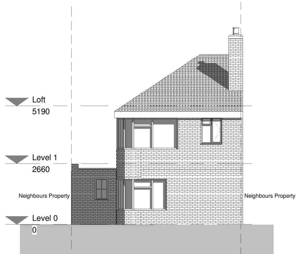
1 Front elevation - Existing
