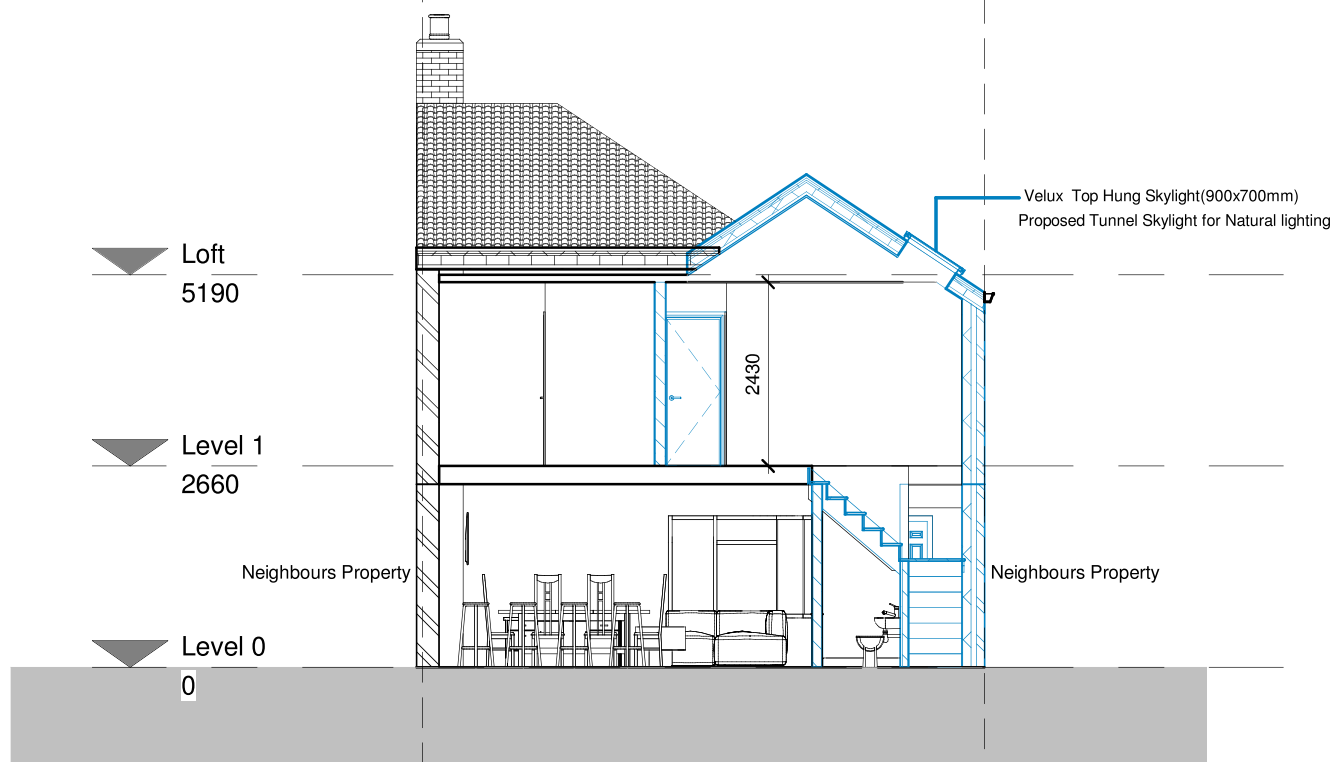
3 Proposed - Section 1 1 : 100
