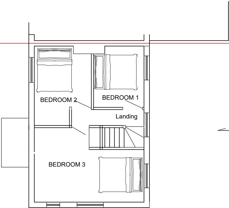
EXISTING FIRST FLOOR. SCALE 1:100.
