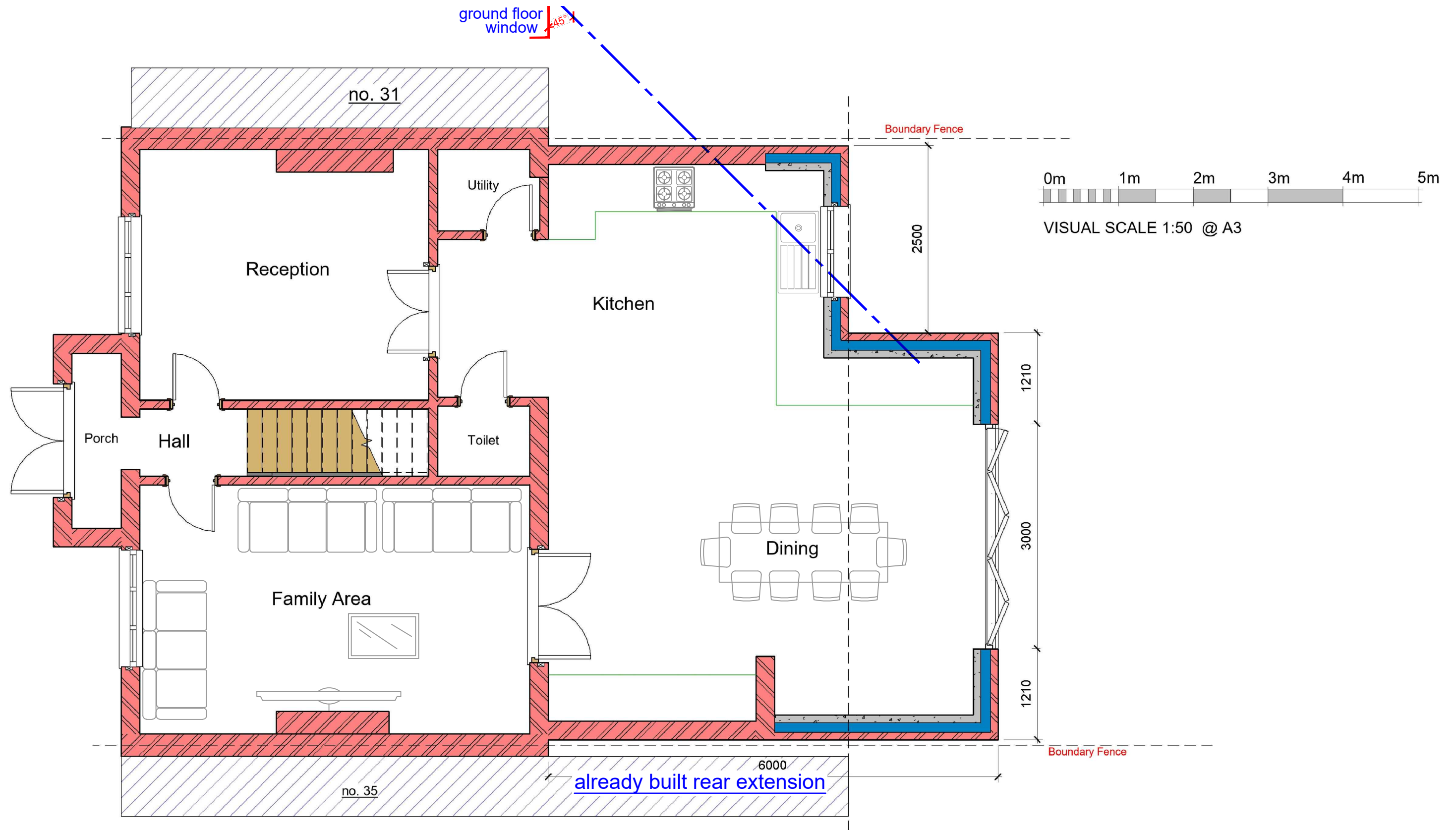
1 Proposed Ground Floor 1 : 50
