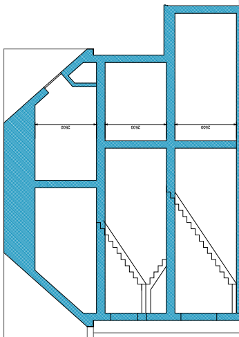
Proposed Section A-A Scale 1:100
