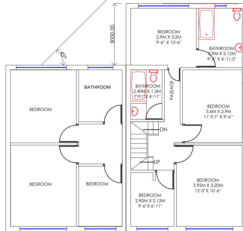
NEIGHBOURING FIRST FLOOR PLAN No. 39
