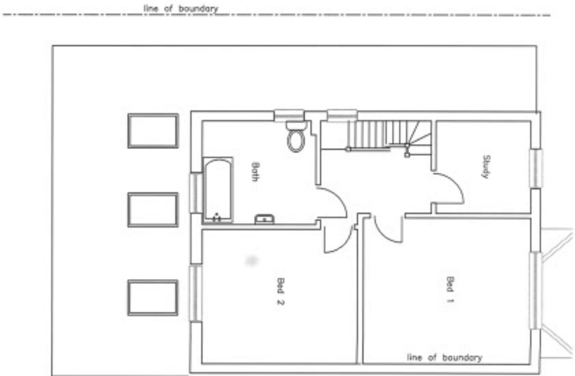
First floor plan extg 1:100
