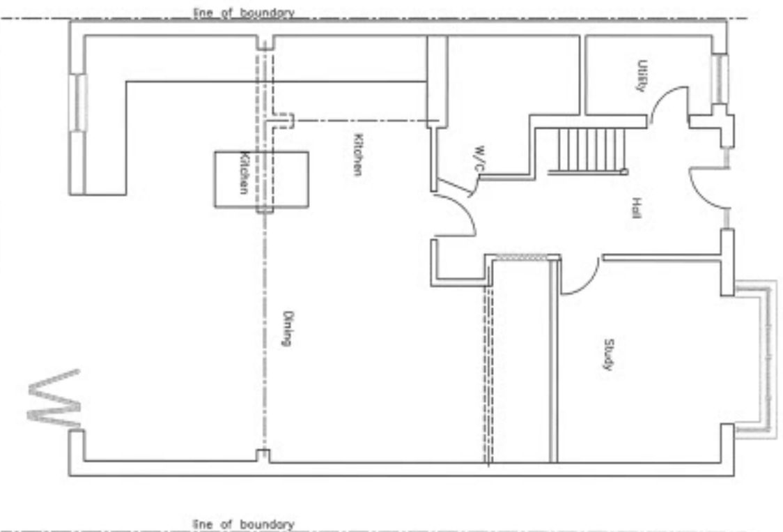
Ground floor plan extg 1:100
