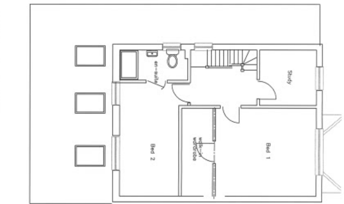
First floor plan extg 1:100
