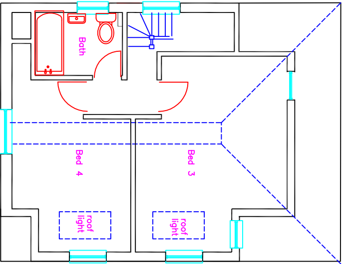
Second floor plan extg 1:100
