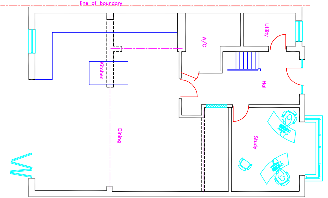
Ground floor plan extg 1:100
