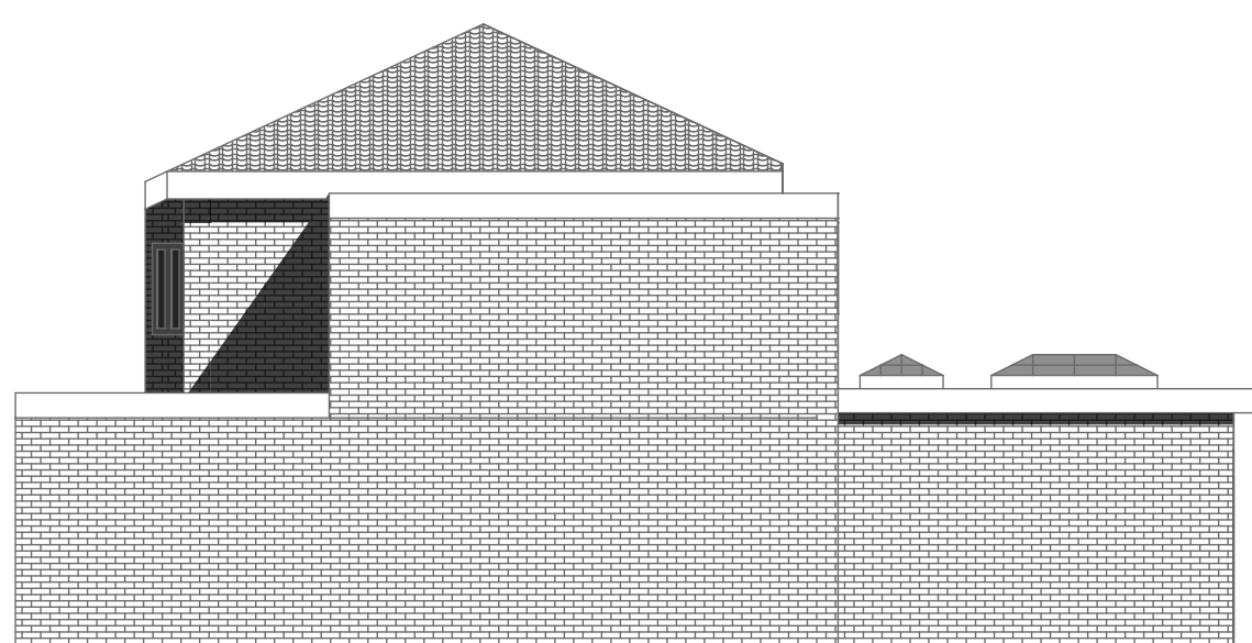
Side Elevation 1 1:100
