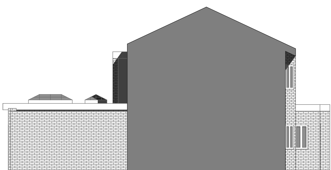
Side elevation 2 1:100
