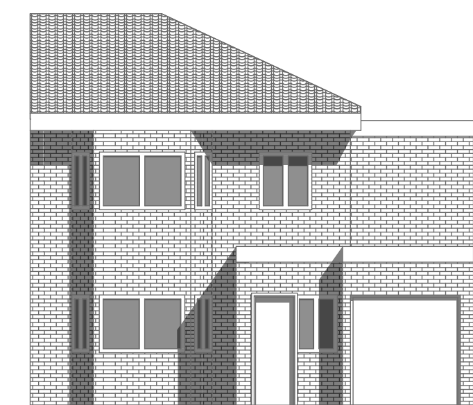
Front Elevation 1:100
