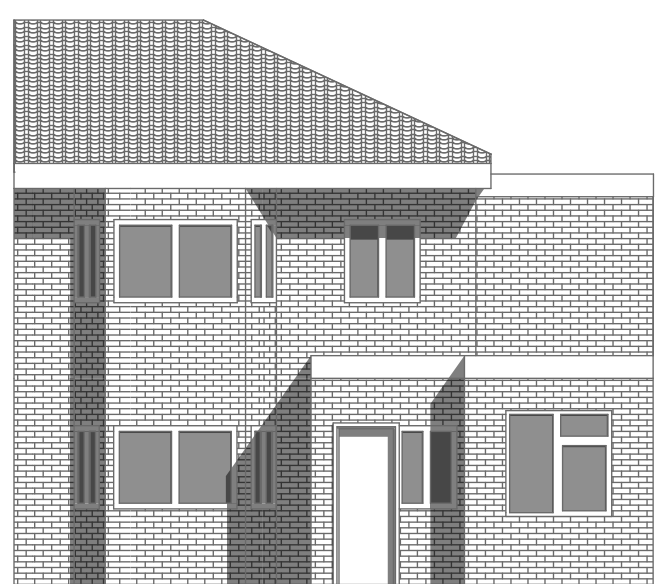
Front Elevation 1:100
