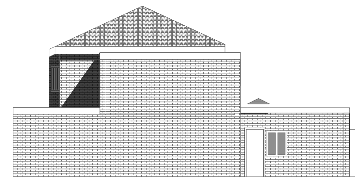
Side Elevation 1 1:100
