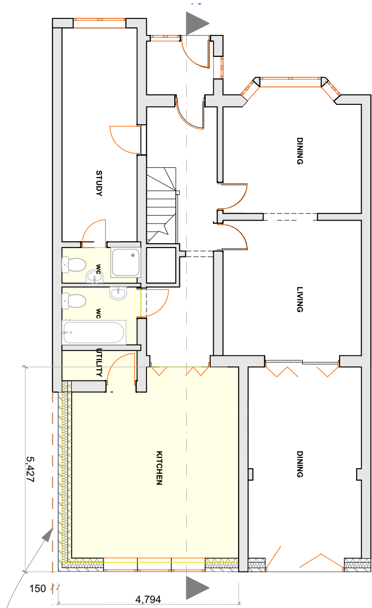
Ground Floor 1:100
