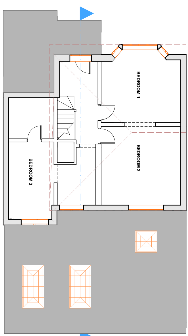
First Floor 1:100
