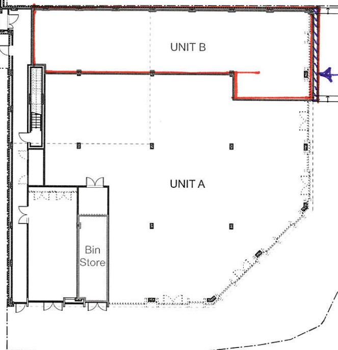
GROUND FLOOR PLAN SCALE 1:250 (at A3)
