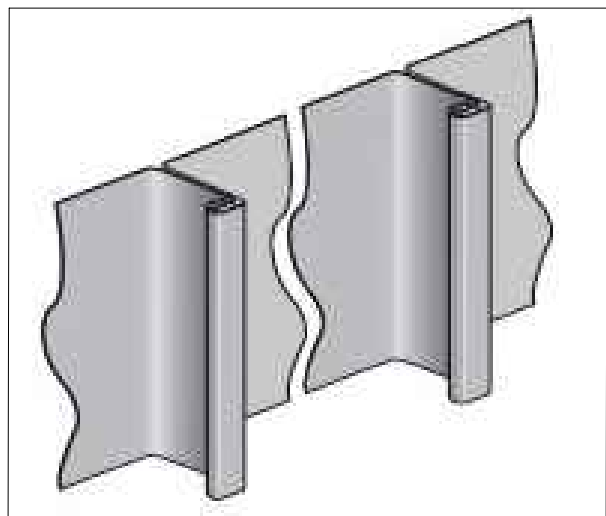
VMZINC - STANDING SEAM PANELS
