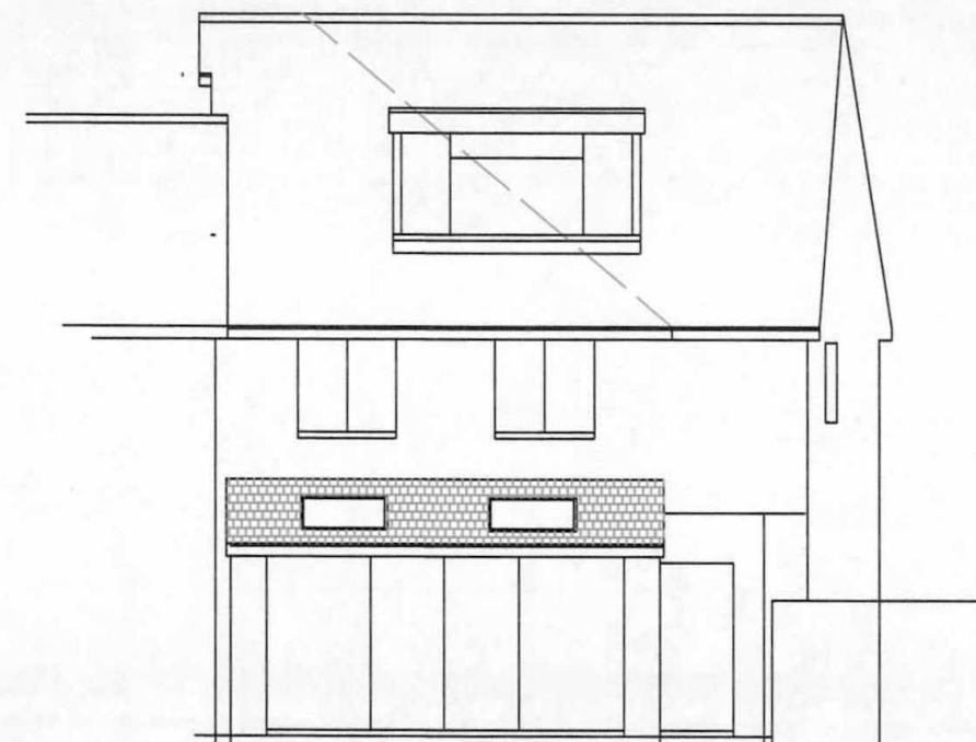
Rear Elevation
