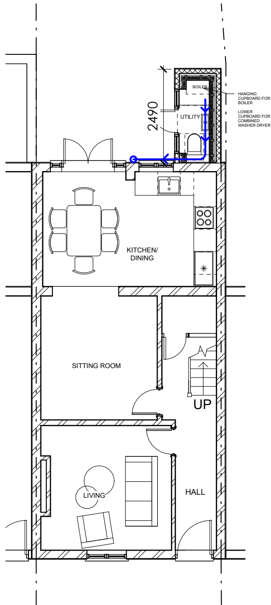
1 PROPOSED GROUND FLOOR PLAN
