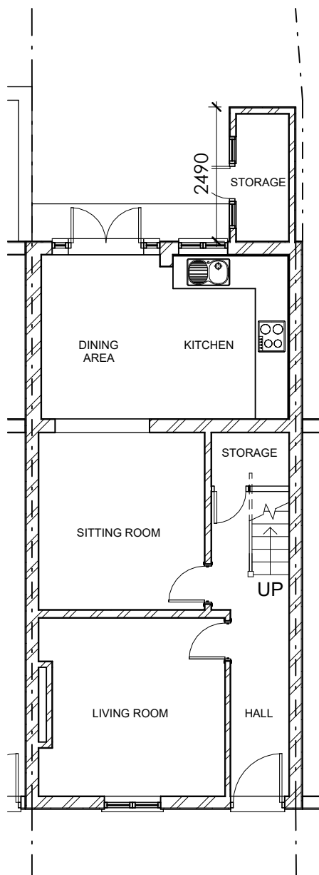
1 EXISTING GROUND FLOOR PLAN
