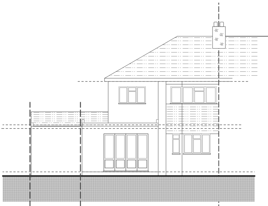
REAR ELEVATION
