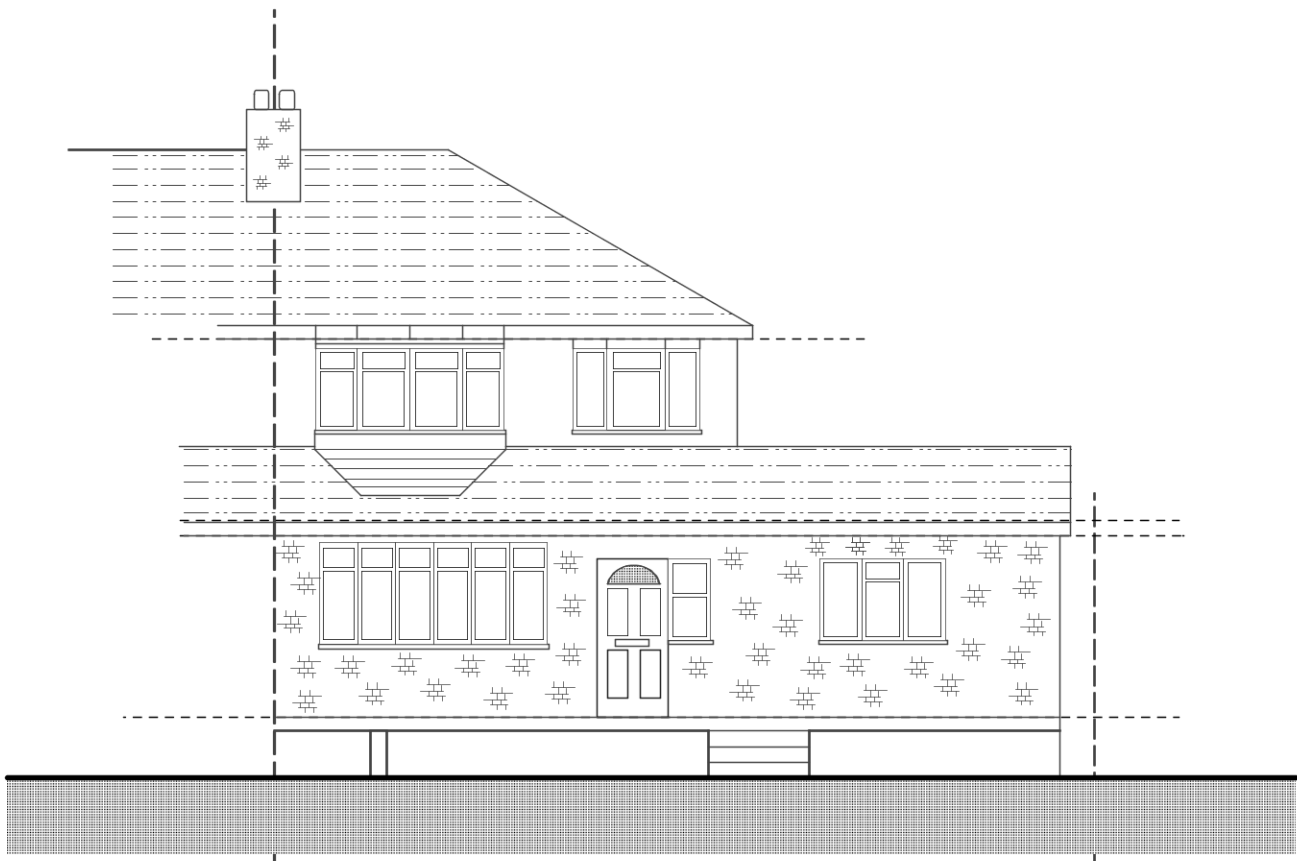
FRONT ELEVATION
