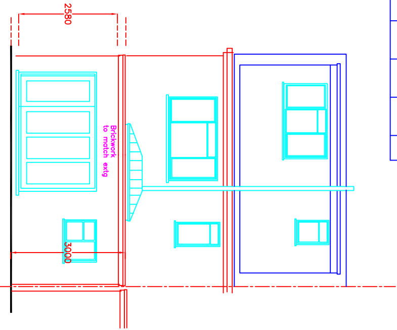
Rear elevation 1:100
