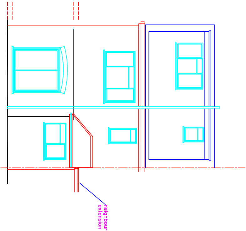
Rear elevation extg 1:100
