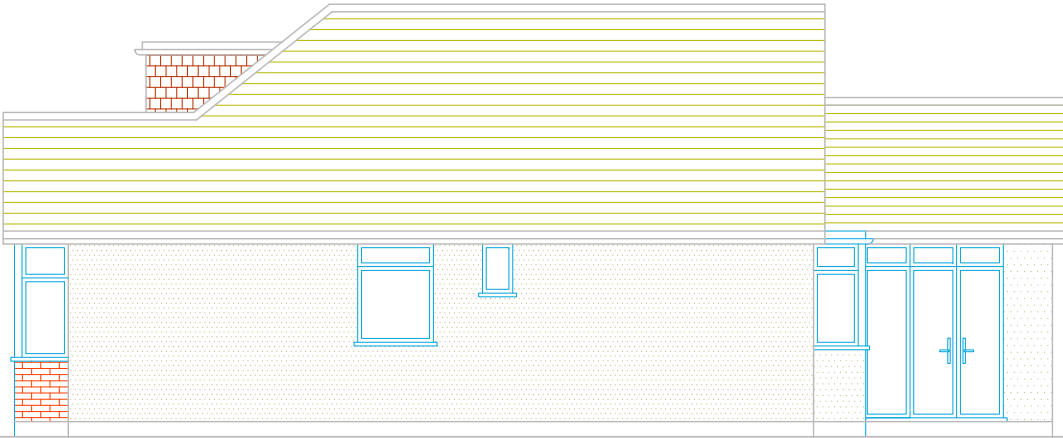
EXISTING SIDE ELEVATION-1
