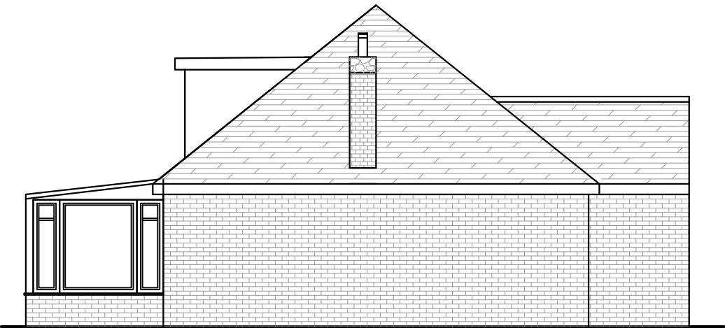
PROPOSED ELEVATION SIDE B
