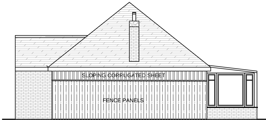
PRE-EXISTING ELEVATION SIDE A
