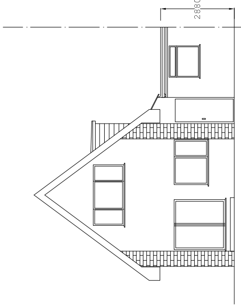
REAR ELEVATION (Existing)
