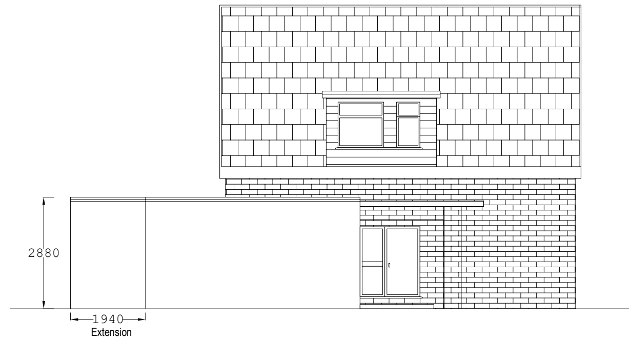
RIGHT SIDE ELEVATION (Proposed)
