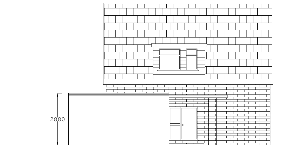
RIGHT SIDE ELEVATION (Existing)
