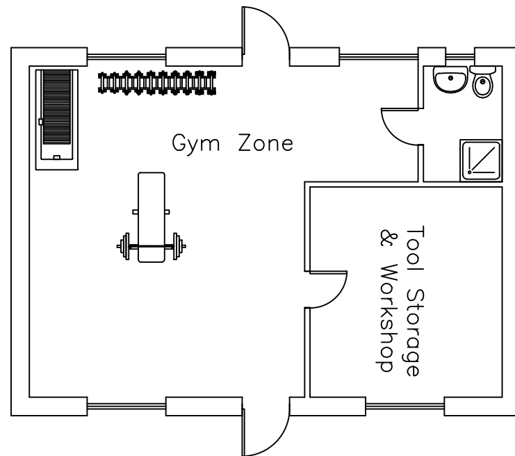
Internal Layout
